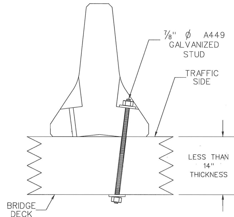
TYPE IV FOUNDATION TYPICAL BRIDGE DECK LESS THAN 14" THICKNESS
