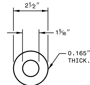
PLAIN GALVANIZED STEEL WASHER FOR 1 1/4" PIN
